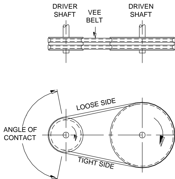
Figure No. 1. Twin vee-belt drive arrangement.
